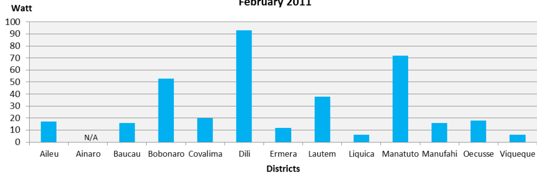
Comparison of Consumption of EDTL-Electricity per Person by Districts February 2011
