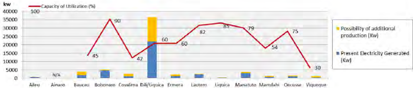
Comparison of Generation of Electricity by EDTL 15 February 2011
