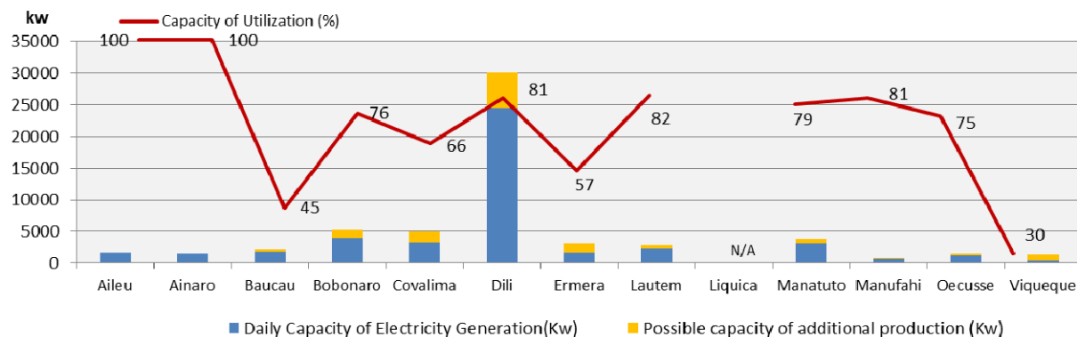
Comparison of Generation of Electricity by EDTL 15 May 2011
