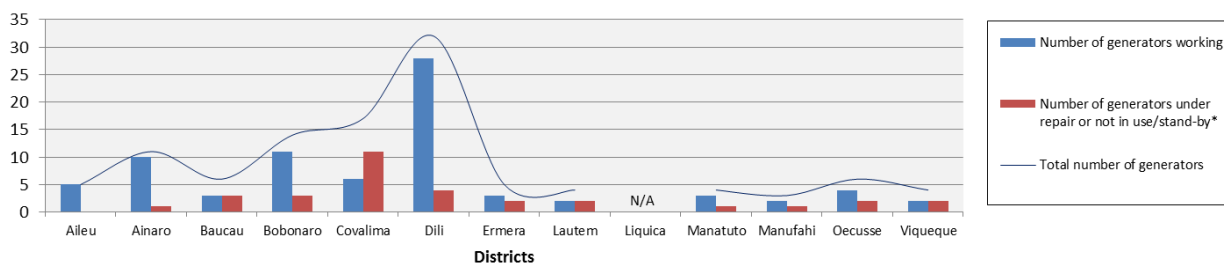
Number of EDTL Generators by Districts May 2011
