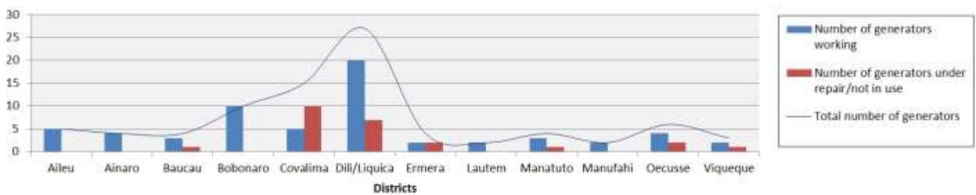
Number of EDTL Generators by Districts December 2010
