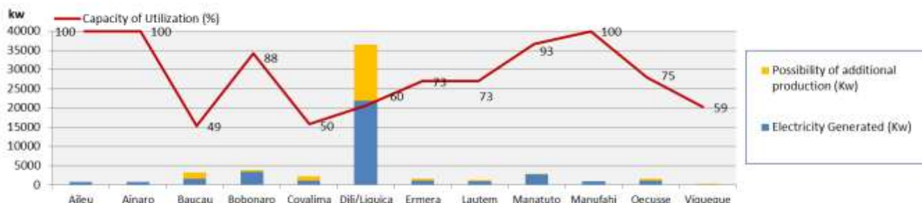
Comparison of Generation of Electricity by ECTL 15 December 2010
