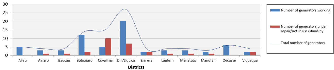
Number of EDTL Generators by Districts January 2011
